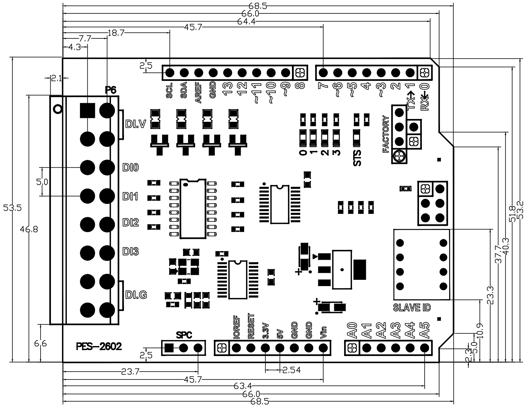
PES-2602 Dimension (mm)
