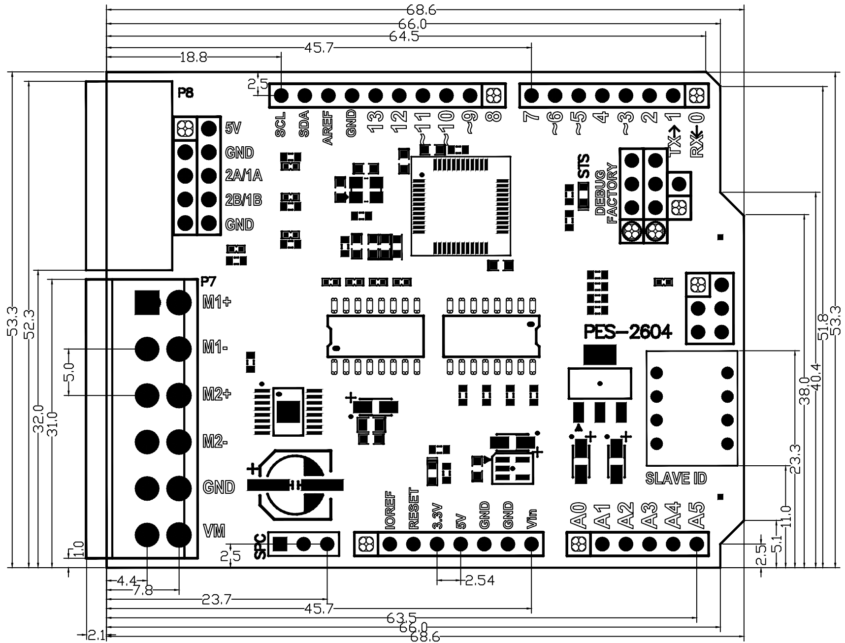
PES-2604 Dimension (mm)
